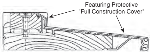
Standard – Aluminum Sill (Inswing) – Mill Finish with adjustable hardwood threshold
