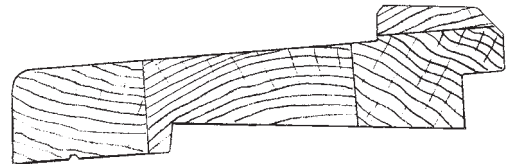
Oak Sill – Laminated (Inswing)
