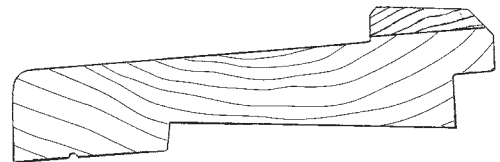
Oak Sill – Solid Base (Inswing)
