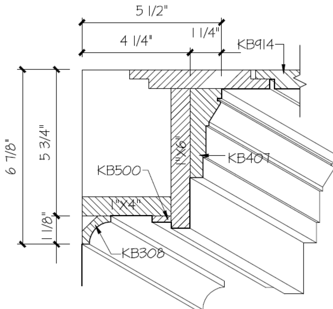
WALL BEAM
