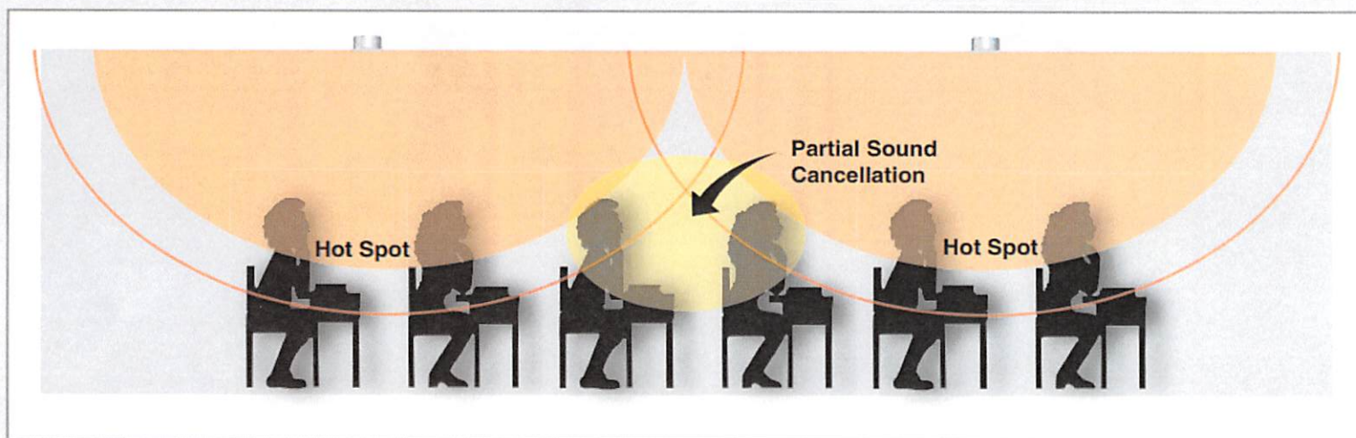
Coverage pattern of a typical ceiling speaker showing hot spots and areas of cancellation.
