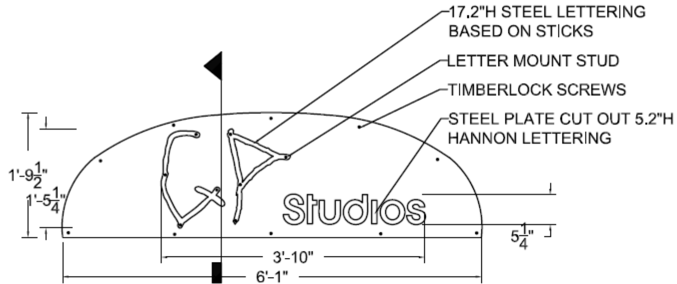
ELEVATION DETAIL
